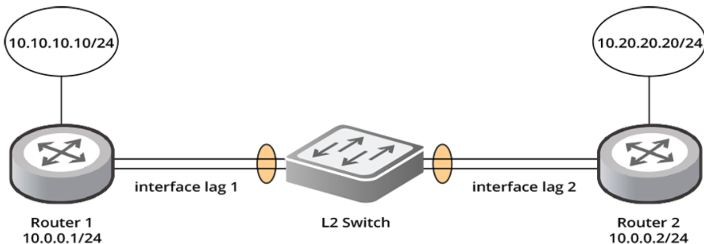
FIGURE 37 Single-Hop BFD Session for One Member Link
