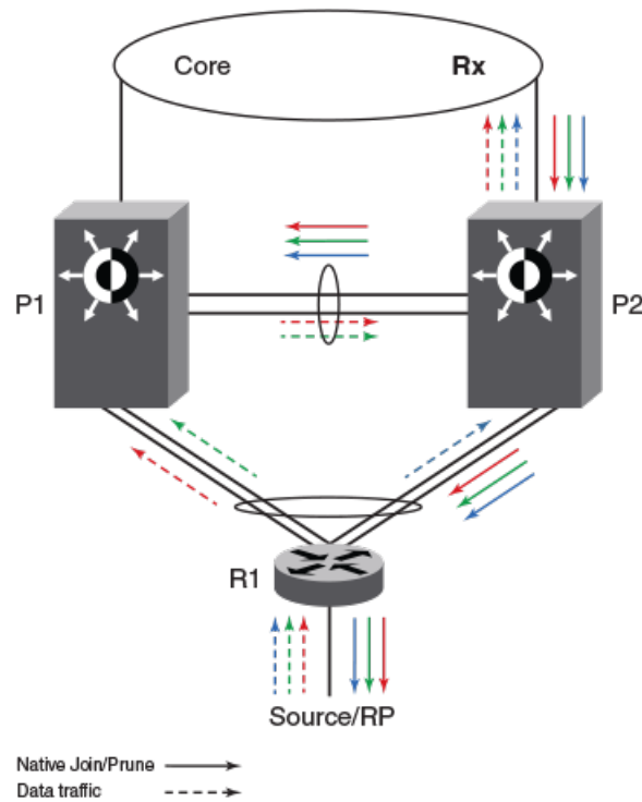
FIGURE 41 MCT Peer as Intermediate Downstream Router
